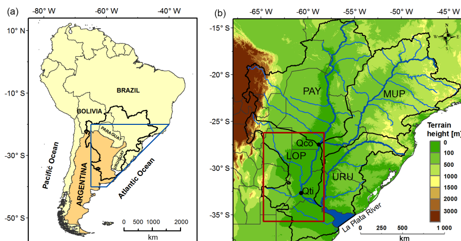
Figure 1. (a) South America and the domains of the La Plata Basin (bold black contour) and southeastern South America (blue polygon). (b) Topography map of La Plata Basin and its subbasins (black contours), Paraguay (PAY), Mid–Upper Paraná (MUP), Lower Paraná (LOP) and Uruguay (URU). The rivers and their tributaries are plotted in blue contours. Gauging stations of the Paraná River streamflow in Corrientes (Qco) and Timbúes (Qti) are highlighted. The study area in northeastern Argentina is highlighted with a red rectangle.
