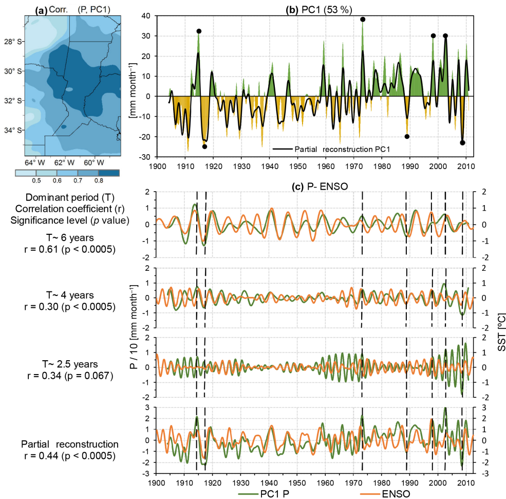
Figure 3. First leading pattern of the 18 m low-pass-filtered precipitation anomalies. Panel (a) shows the spatial distribution of the correlation between PC1 (in b) and each precipitation time series at a single grid point. The percentage of explained variance is given in brackets. Panel (c) compares the time series of the dominant cycles of the PC1 of SSTs related to the ENSO pattern and regional precipitation at interannual timescales. Precipitation modes have been scaled to facilitate their interpretation. Vertical dashed lines coincide with months of maximum wet anomalies and the severest droughts (dots in b). Significance levels (p values) for the Pearson correlation coefficients (r) are estimated by combining 2000 Monte Carlo iterations considering autocorrelation by resampling in the frequency domain (Macias-Fauria et al., 2012).
