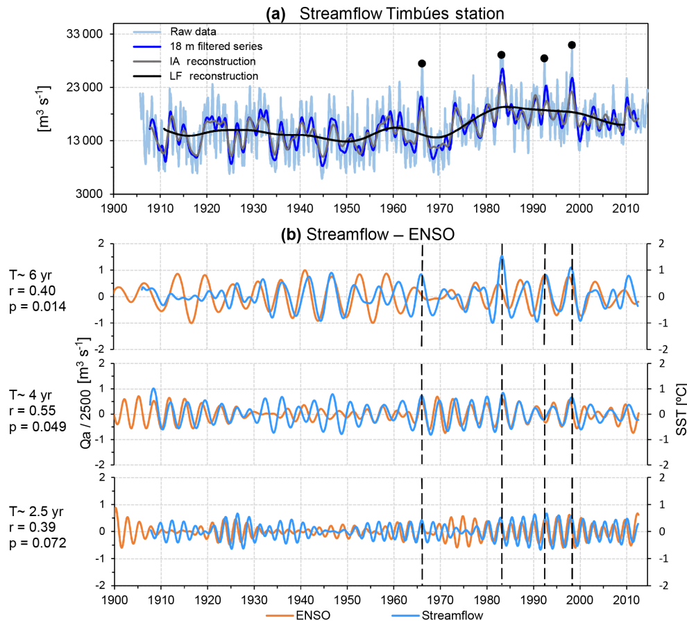
Figure 4. (a) Monthly mean streamflow time series for the Paraná River at Timbúes station and its partial reconstruction using all significant modes of interannual (IA reconstruction) and decadal-to-multidecadal variability (LF reconstruction) presented in Table 2. (b) Time series of the dominant modes of Paraná River streamflow anomalies and the ENSO pattern on interannual timescales. Streamflow modes have been scaled to facilitate their interpretation. Dominant periods ( T ) of the leading modes and Pearson correlation coefficients ( r ) together with their significance levels ( p ) are given to the left of the figure. Significance levels ( p values) for r are estimated by combining 2000 Monte Carlo iterations considering autocorrelation by resampling in the frequency domain (Macías-Fauria et al., 2012). Vertical dashed lines coincide with extreme flood events in 1966, 1983, 1992 and 1998.
