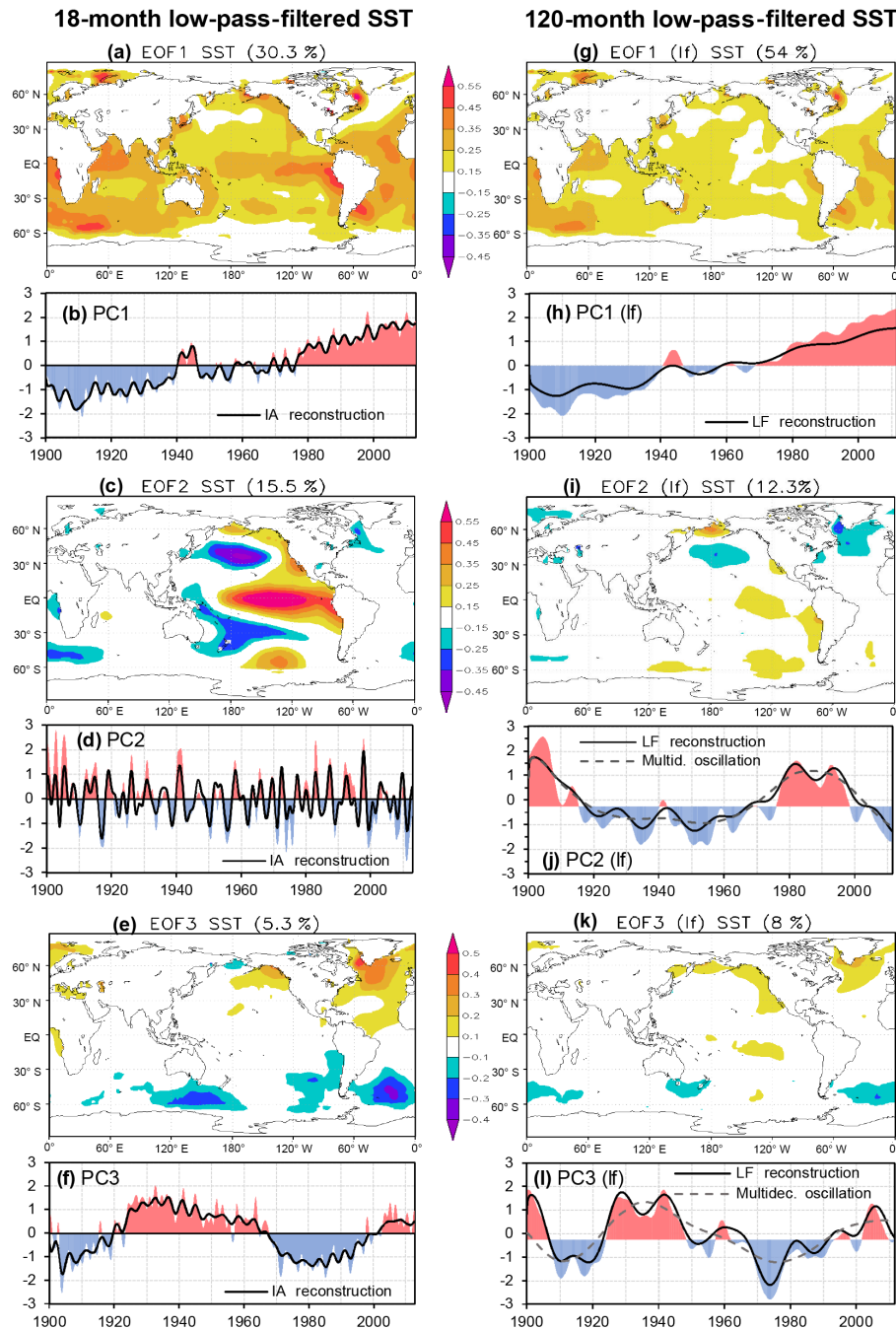
Figure 2. First three leading global pattern of 18- and 120-month low-pass-filtered monthly mean SST between January 1901 and September 2012. Patterns are described by the spatial loadings (EOFs) and their associated PCs. The percentage of variance explained by each pattern is given in brackets. The original time series are partially reconstructed using the significant components detected with SSA. Partial reconstructions at interannual timescales are plotted in PCs of the left column (IA reconstruction). Partial reconstructions at low-frequency timescales (LF reconstruction) are plotted in PCs (lf) of the right column. The partial reconstructions include all variability modes at each timescale shown in Table 1. Panels (j) and (l) also show the multidecadal oscillations.
